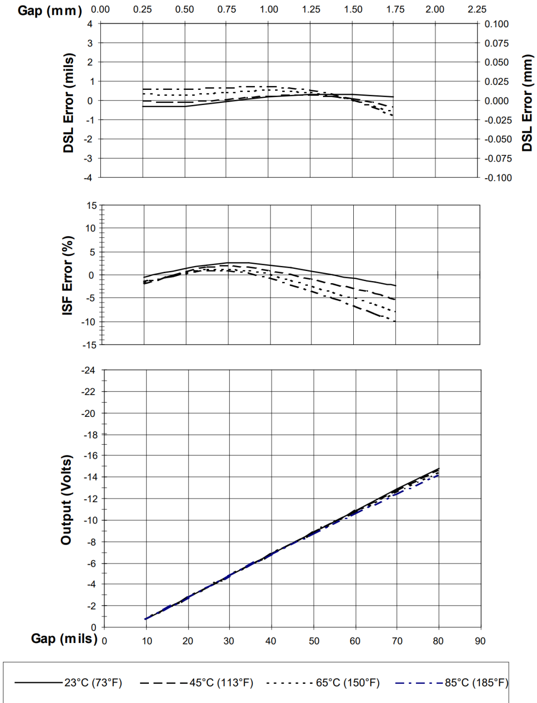
Figure 8: Typical 3300 XL NSv 7 m Proximitors Sensor with 6 m of Extension Cable @ High Temperature (Probe is at 25°C)
